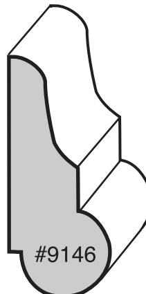
#9146 3/4" x 1-3/4"
